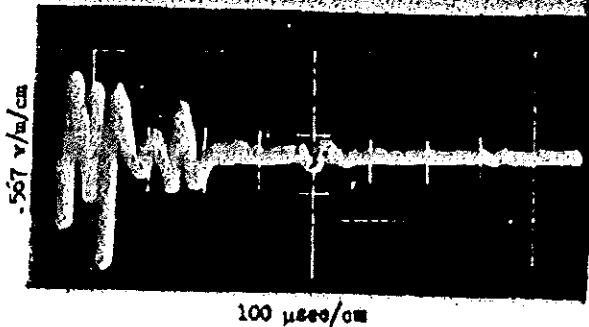
Fig. 3.62 Broadband pulse Shot No. 2 1000 km from ground zero
